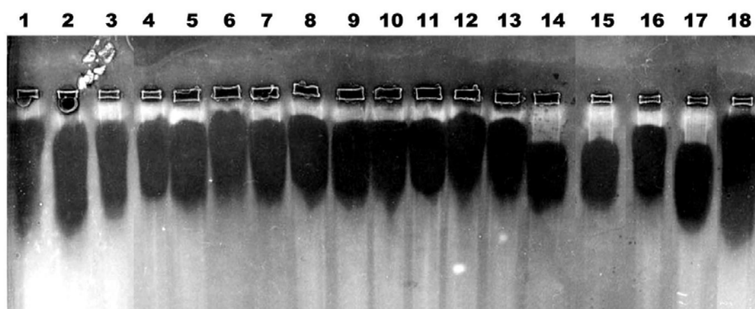
Fig. 6. Zymogram patterns of isolates of Fusarium culmorum . Lanes 1-13, ZP10; lanes 14-15, ZP10; lane 16, ZP10; lane 17, ZP9; lane 18, ZP10. Lanes 1, 2, 5, 6, 7, 8, 10, 11, 14, 15, 16, & 17 potato isolates; lanes 3 & 4 bean isolates; lane 9 onion isolate; lanes 12 & 13 tomato isolates and lane 18 wheat isolate
