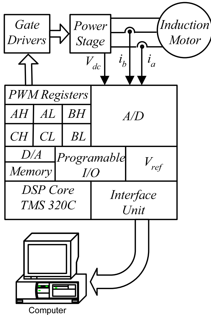
Fig. 9. Experimental setup
