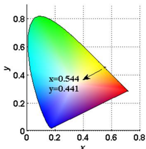
Fig. 6. CIE 1931 coordinates diagram for curcumin OLED light spectrum
