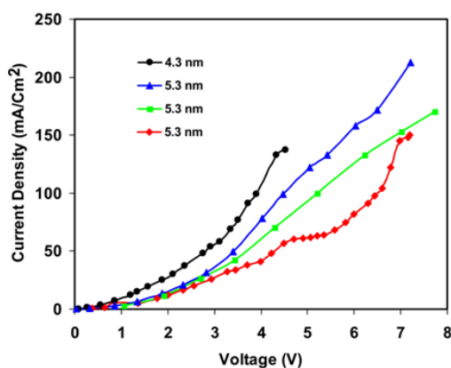
Fig. 7. The Current Density ( J ) versus voltage ( V ) for curcumin OLED
