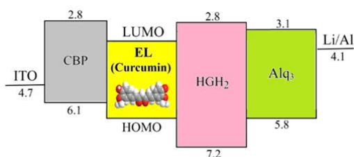
Fig. 4. Schematic energy level (in eV) diagram of multi-layer fabricated OLED using curcumin
