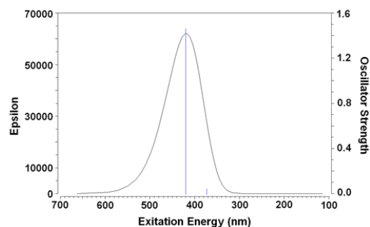
Fig. 11. TD-DFT calculated UV-Vis spectrum for curcumin obtained at B3LYP/6-311G (d,p) level of theory
