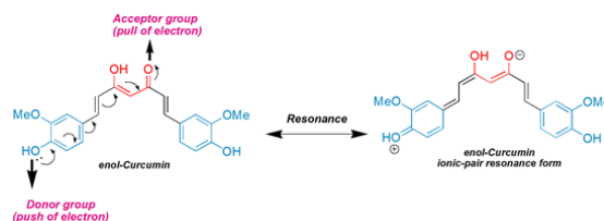
Fig. 10. Push-pull effect through conjugated bonds in curcumin
