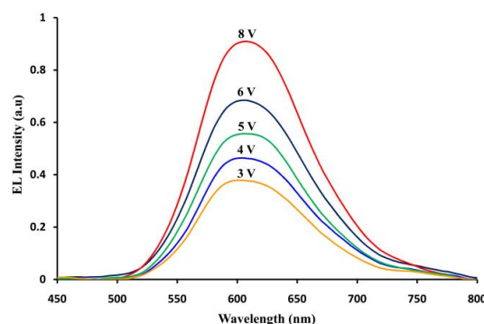
Fig. 5. Normalized EL spectra of curcumin OLED with a non-doped emissive layer
