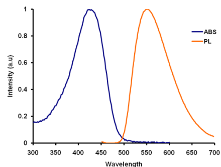
Fig. 3. ABS and PL spectra of curcumin in MeOH
