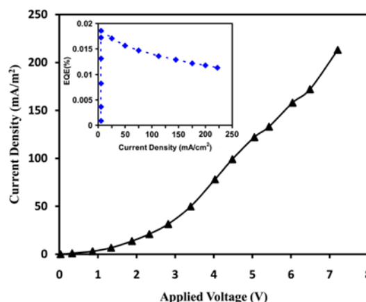
Fig. 8. Current density J as a function of the voltage V and external quantum efficiency (EQE) of device as function of J
