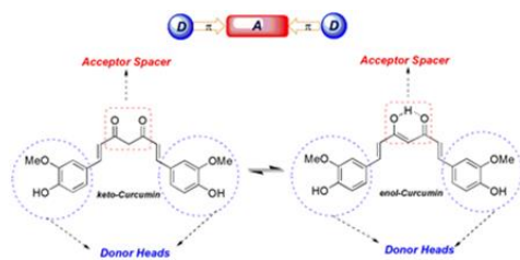
Fig. 2. The chemical structure of two curcumin's tautomers as D-A-D chromophores
