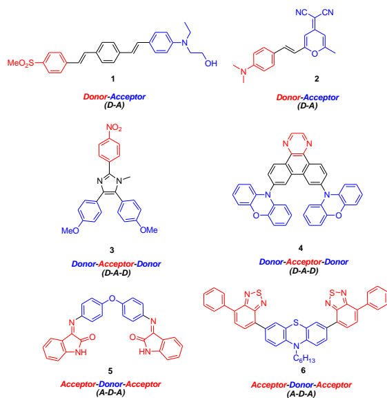
Fig. 1. The chemical structure of some D-A, D-A-D and A-D-A chromophores
