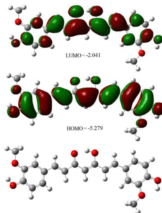
Fig. 9. Optimized molecular structure for the most stable form of curcumin, and its HOMO and LUMO surfaces beside their calculated energies (in eV) at B3LYP/6-311G (d,p) level of theory
