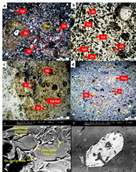
Fig. 3. Photomicrographs (a, b, c, d) of loess samples. (a) Loess sample from Gundar village (MAL 8) in Maravehtappeh region: crystals of quartz within clay coating, k feldspar, and carbonates. (b) Wide distribution of tourmaline + biotite + sphene + chlorite + gypsum (DL 20 sample). (c) A typical zircon (from Polyolia village; MAL 19) with tetragonal structure, metamicticity rim and pyramidal surfaces at the end of the cross section (d) Assembly of quartz and zircon in the clay coatings in a loess samples from Gorgan area (OG 4). (e) Conchoidal fractures and crystalline nodules with overgrowth texture in quartz grains. (f) A typical crystal of altered zircon with tetragonal structure. Mineral abbreviations: Qz= quartz, Kf= K-feldspar, Zr= zircon, Dol= dolomite, Chl= chlorite, Tur = tourmaline, Gs= gypsum, Bt= biotite, Spn= sphene and Cal= calcite
