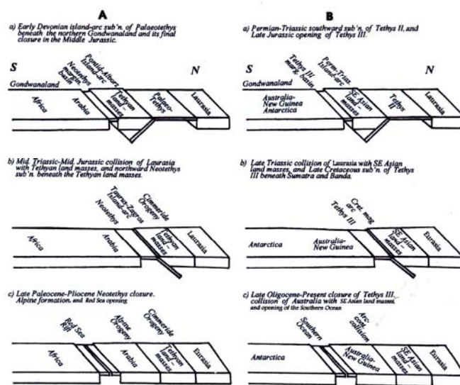
Fig. 2. Comparison of tectonic evolution of the Tethyan (A), and SE Asian Regions (B). Arc. Cont collision=Arc-continent collision; Cret. mag Arc=Cretaceous magmatic arc; Marg. basin=marginal basin
